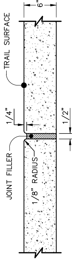
TRANSVERSE EXPANSION JOINT
