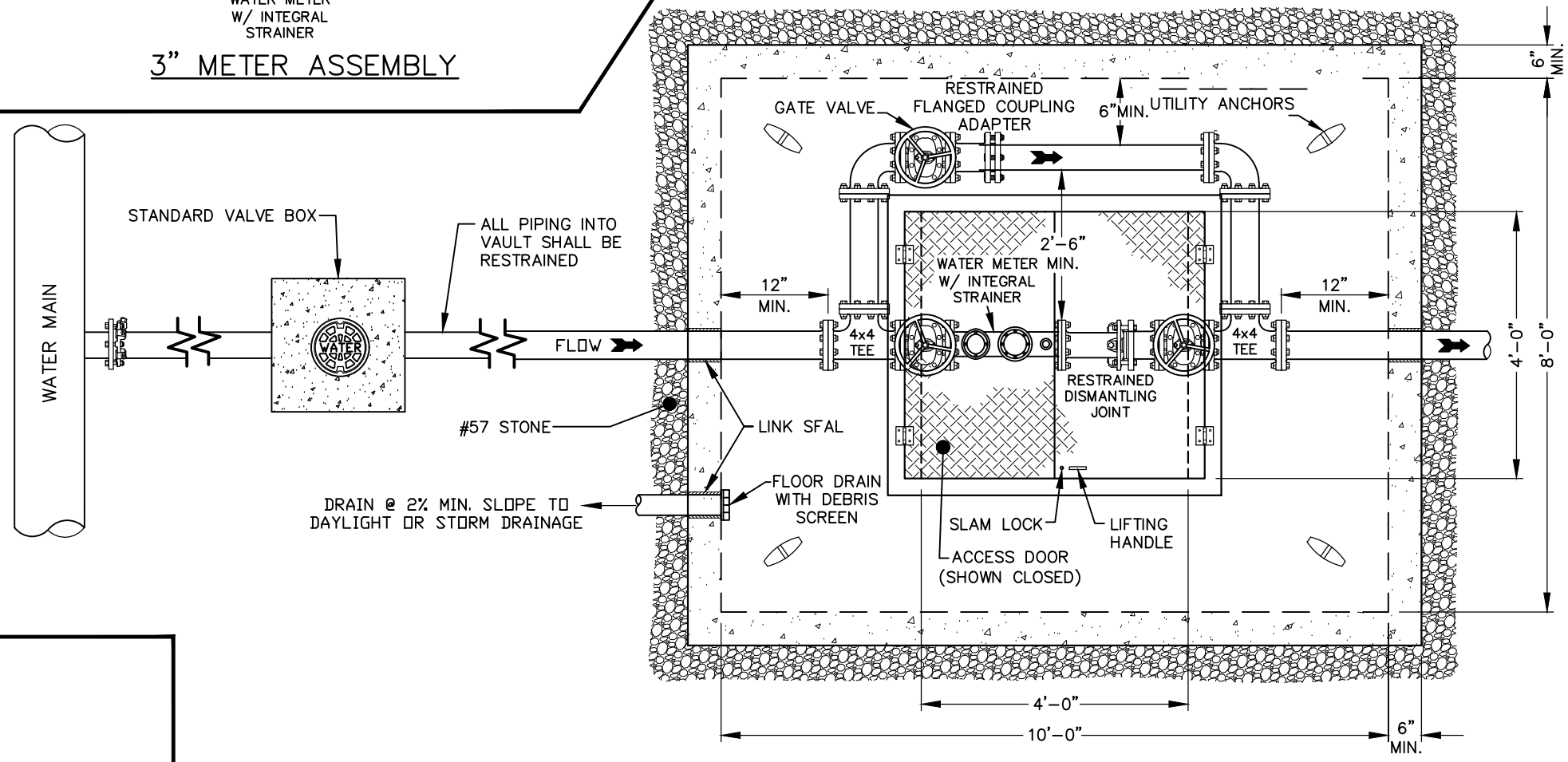
PLAN VIEW
