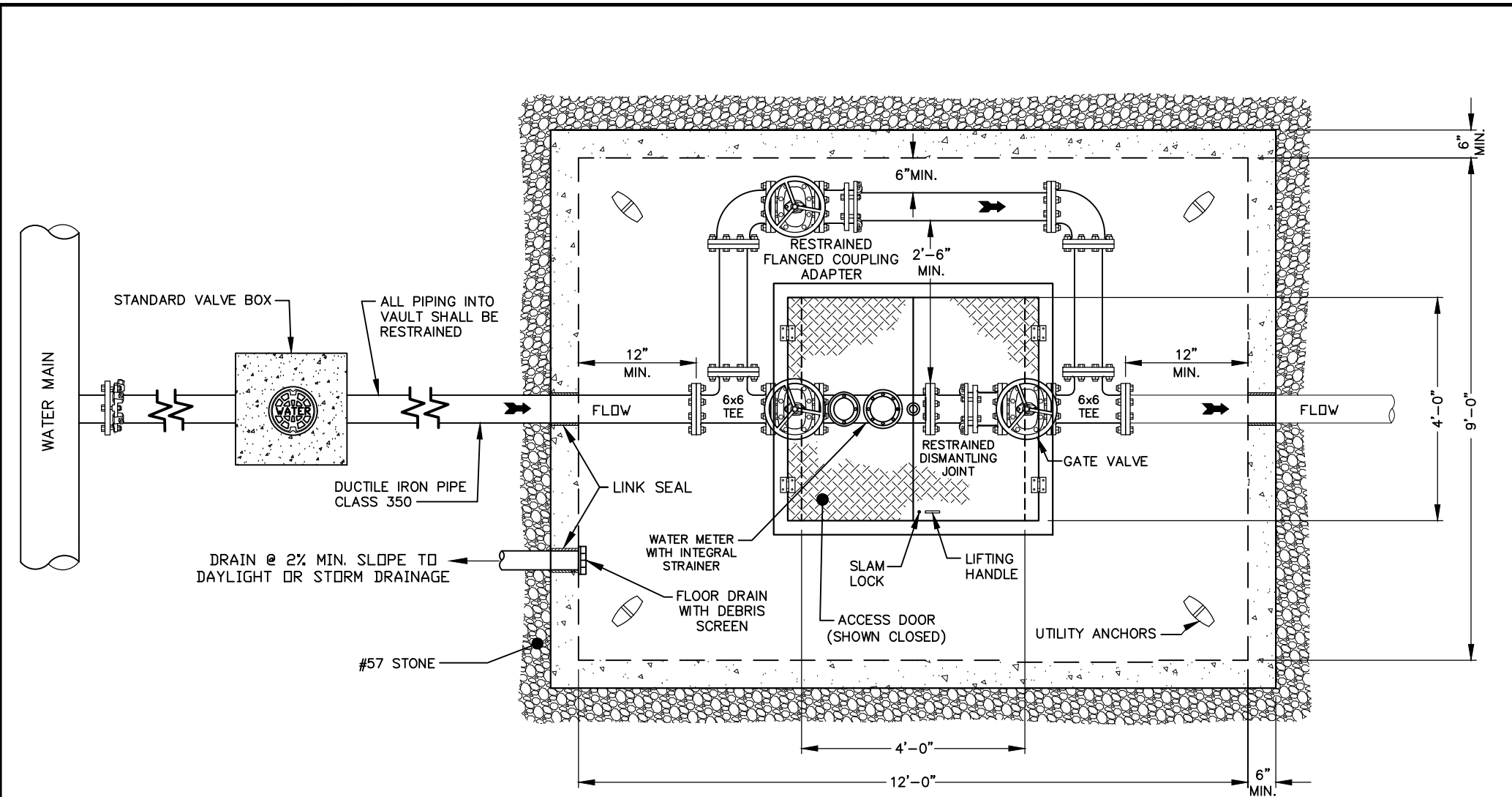
PLAN VIEW
