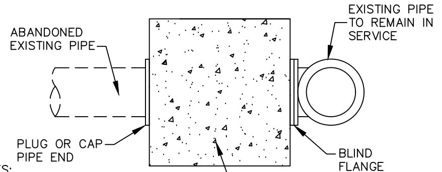
B. TYPICAL IN-LINE PIPE CUT AND RESTRAINED PLUG
