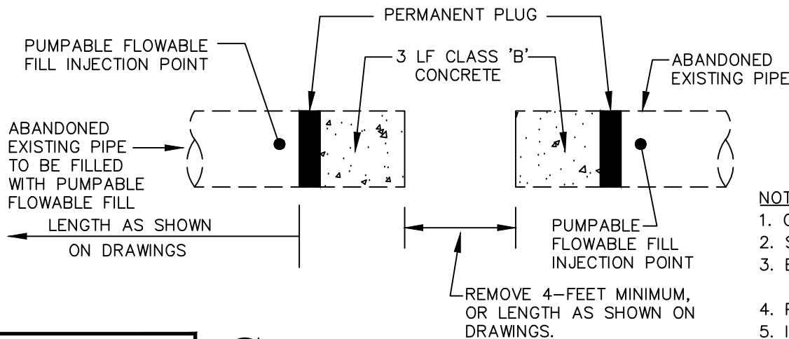
C. TYPICAL IN-LINE PIPE CUT AND PLUG
