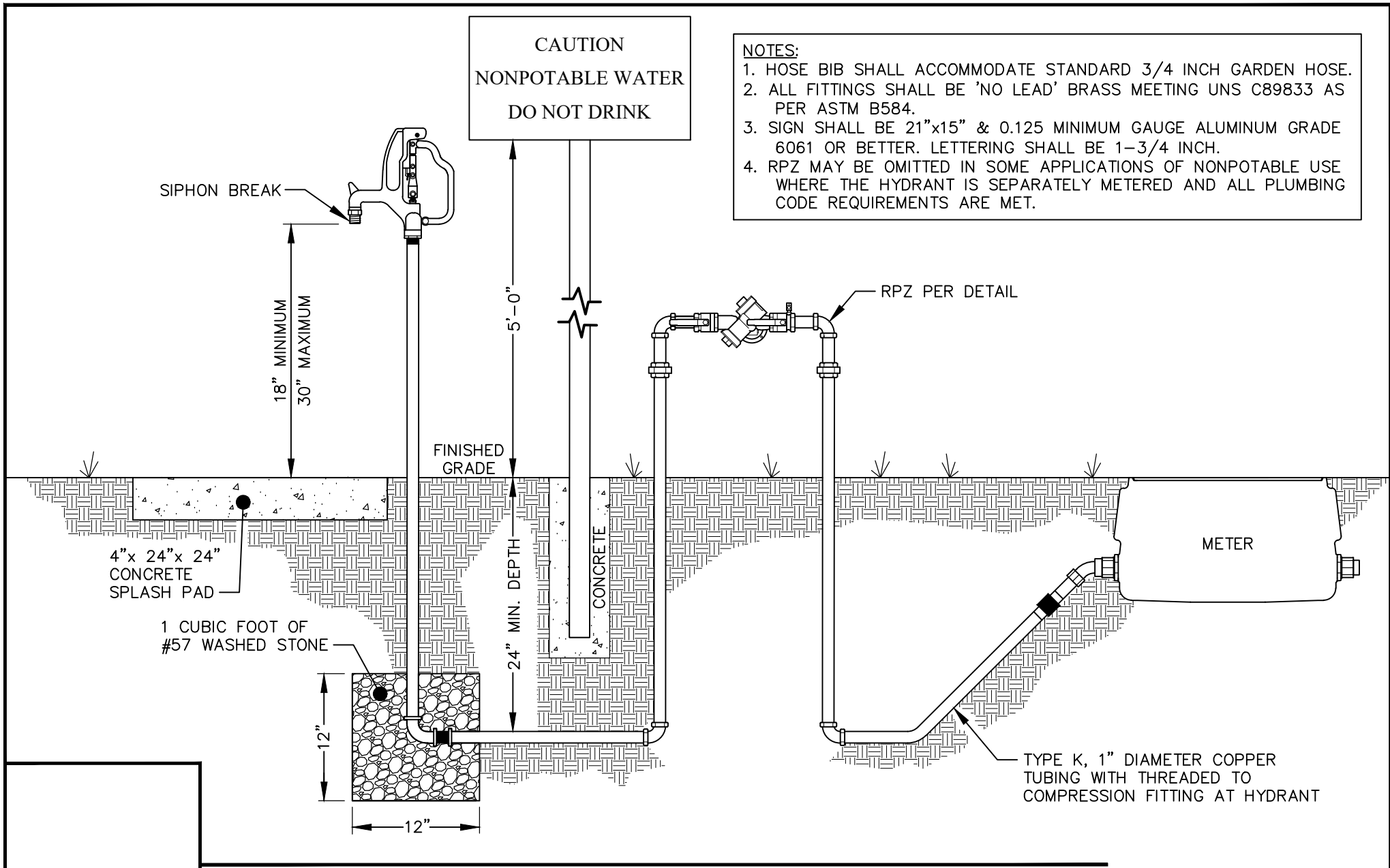
STANDARD YARD HYDRANT (NON-FREEZE)
