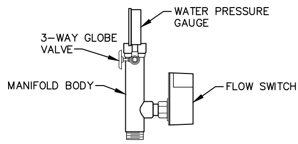
RISER MANIFOLD SIDE VIEW
