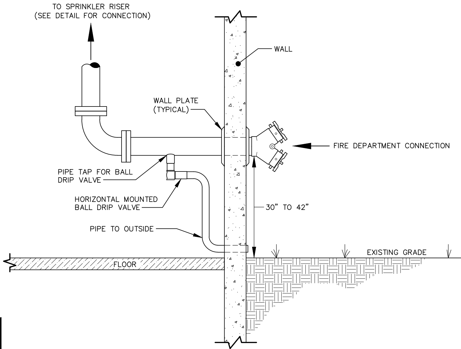
WALL MOUNTED FIRE DEPARTMENT CONNECTION
