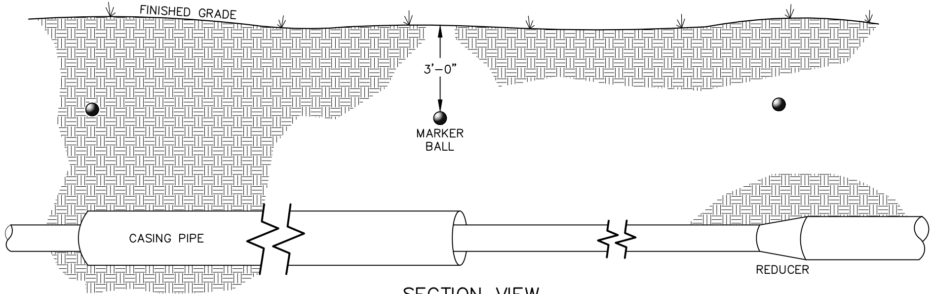
SECTION VIEW
