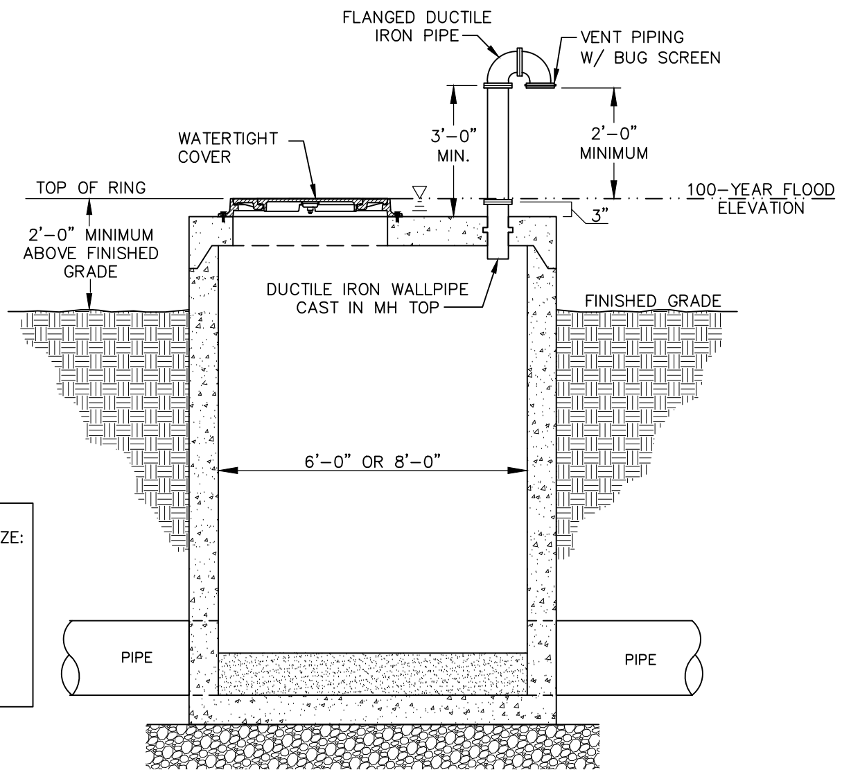
SECTION VIEW
