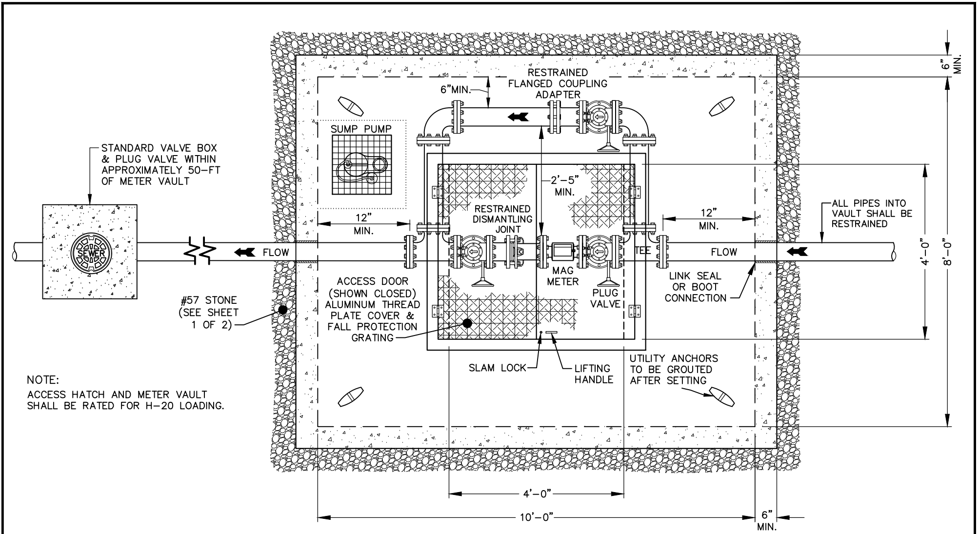
PLAN VIEW (SEE SHEET 1 OF 2 FOR SECTION VIEW)
