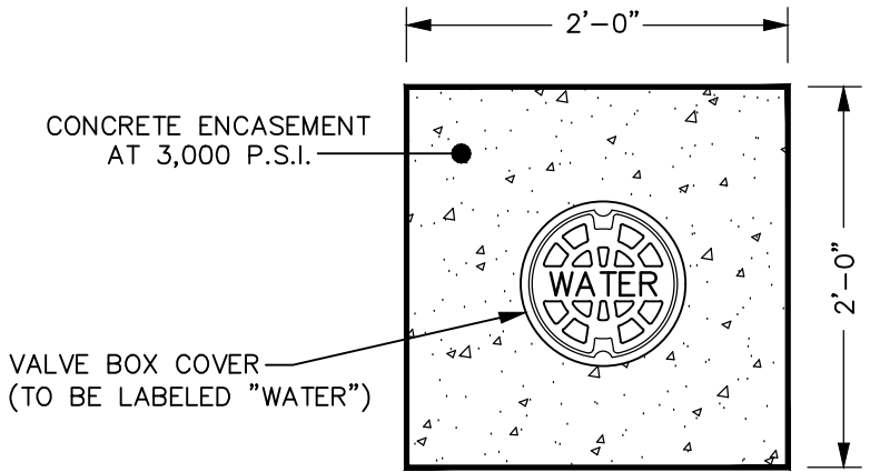
PLAN VIEW FOR UNPAVED AREAS
