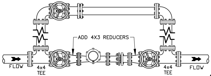
3" METER ASSEMBLY
