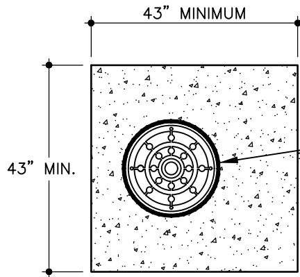
CONCRETE SLAB
